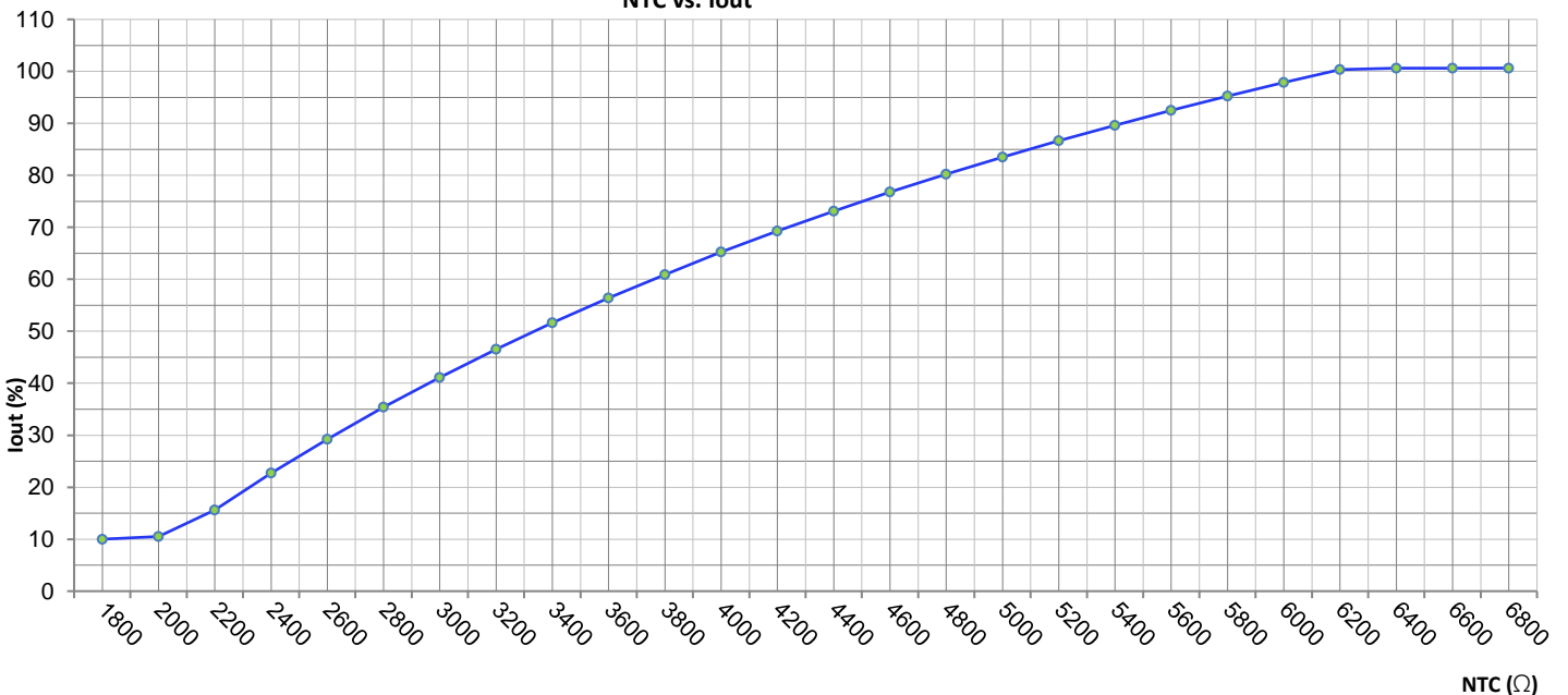
NTC vs. Iout
